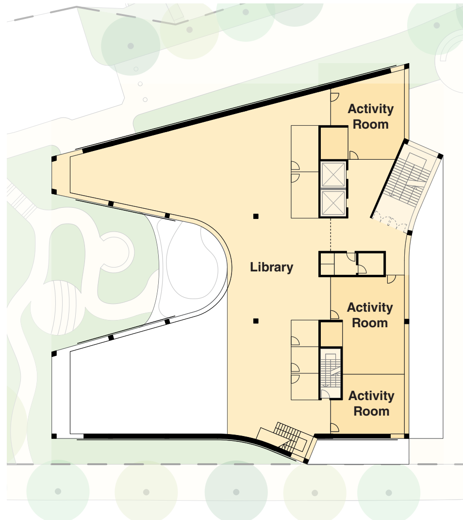
Level 2 Plan
